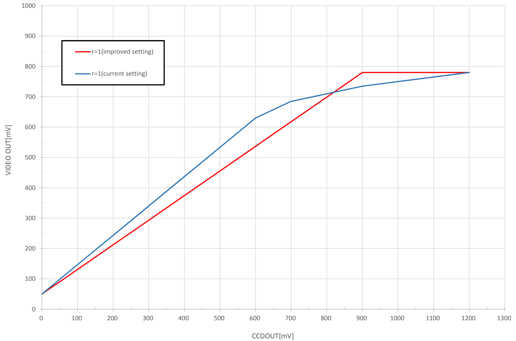
WAT-910HX r=1 Characteristics
